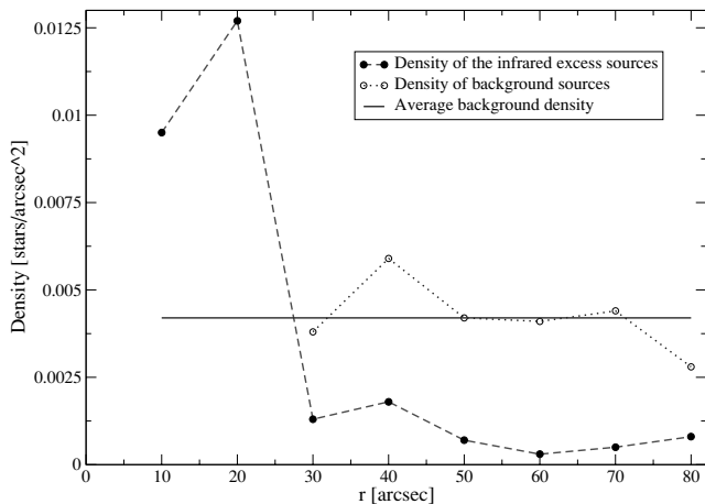
Figure 2. Projected stellar density around \alpha_{2000} = 10^{\text{h}}45^{\text{m}}53^{\text{s}}.6 , \delta_{2000} = -59^{\circ}57'02'' . Dashed and dotted lines refer to the density of IR excess and background (i.e. with and without IR excess) sources, respectively. The average background density seems to have a constant value of about 0.0042 \text{ stars arcsec}^{-2} and is represented by a solid line.
