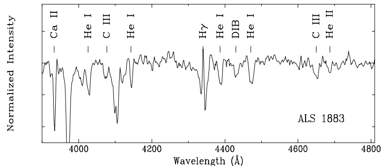
Figure 5. Normalized blue spectrum of LS 1883 obtained at CASLEO. The O9.5V spectral classification is derived from the presence of He II 4686 Å, and the barely visible He II 4541-Å absorption lines compared with He I 4471 Å, and also from the moderately strong C III 4650-Å absorption line.
