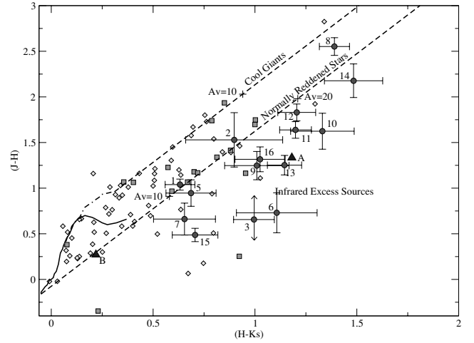
Figure 3. The JHK_s C–C diagram for an 80-arcsec field centred in \alpha_{2000} = 10^{\text{h}}45^{\text{m}}53^{\text{s}}.6 , \delta_{2000} = -59^{\circ}57'02''.0 . The unreddened main-sequence locus between O3V and M2V is indicated with a solid curve, while the cool giant branch is denoted with a dash-dotted line. The reddening track for normal O3V and cool giant stars are plotted as dashed lines, with crosses indicating A_V = 10 and 20 mag of (normal) visual extinction from the points where they intersect the main-sequence and cool giant curves, respectively. Filled circles refer to IR cluster stars, squares to suspected foreground or background stars between the circles 22.5 and 40 arcsec of radii, diamonds to field stars, and triangles to the luminous optical stars labelled with A (SS73 24) and B (LS 1883). Numbers label the IR sources from Table 1. Error bars represent the possible values within the 95 per cent confidence level, and are plotted only for the IR cluster stars.
