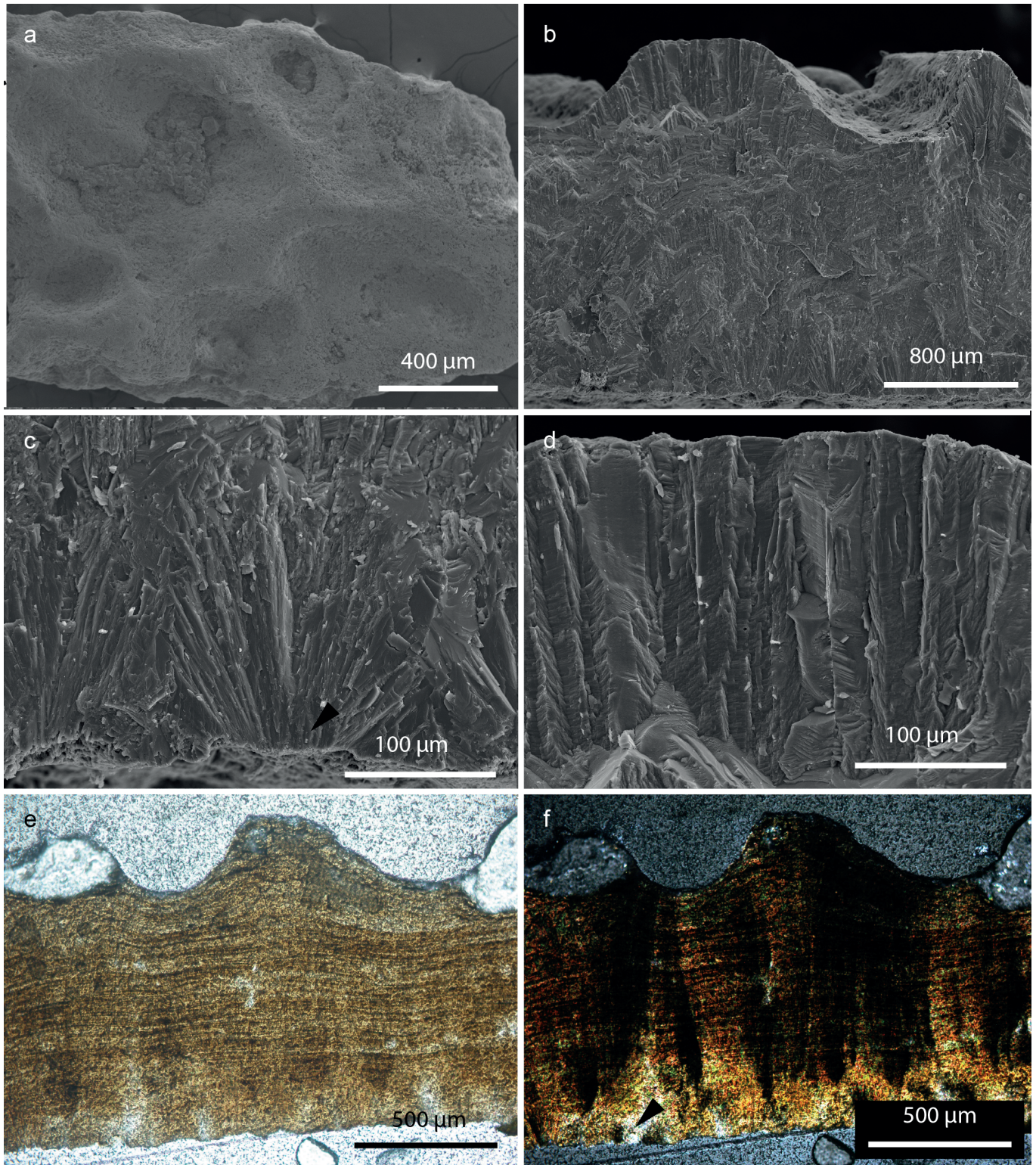
Figure 3. Guegoolithus turoloensis from the El Horcajo site (La Rioja). Scanning electron microscope microphotographs (a-d), petrographic microscope photograph in parallel nicols (e), and petrographic microscope photograph in cross nicols (f). a) MENC- MENC-TREN-13. Outer surface showing sagenotuberculated ornamentation. b) TRE-2. Radial section of the eggshell. c) MENC-TRE-2. Detail of the mammillae showed in a. Note the radial acicular ultrastructure. Black arrowhead points a preserved organic core. d) MENC-TRE-2. Detail of the upper part of the eggshell, showing radial tabular ultrastructure. e) MENC-TREH1. Above the mammillae, the eggshell shows an intense lamination, parallel at the bottom and progressively undulating to the top. f) MENC-TREH1. Observe the undulating extinction. Black arrowhead points a preserved organic core.
