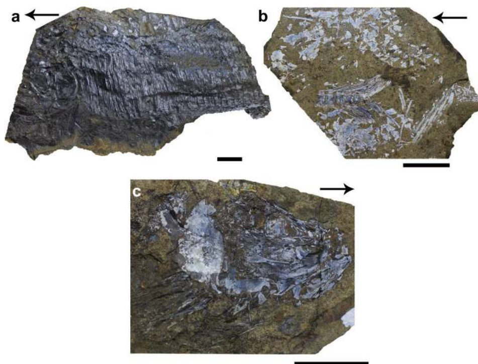
Figure 2. Some of the material recovered in the latest Antarctic field expeditions. (a–c) Material collected at Ameghino Formation. (a) IAA-Pv 424 Aspidorhynchiformes cf. Vinctifer , incomplete specimen in lateral view (b) IAA-Pv 324 Aspidorhynchiformes caudal endoskeleton, bones, and scales, (c) IAA-Pv 368 Teleostei indet. photograph of the head and pectoral fin, Scale bar= 20 mm. Arrow point anteriorly.
