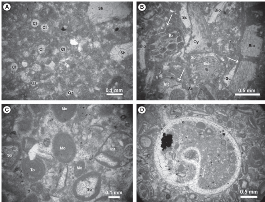
Fig. 6. A, subfacies A1, wackestones to floatstones. Calcispheres (Cl) and shell debris (Sh) immersed in a micritic matrix with quartz fragments (Qz). B, subfacies B1, bioclastic grainstones to rudstones. Various benthic skeletal grains: echinoderm spine (Sp), bryozoan (Br), oyster (Oy), echinoderm plates (Ech) and other bioclastic fragments (Bio) are cemented by sparry calcite (Sc); note that most of the bioclastic fragments and the intraclast (Int) have a micritic coating (arrows). C, subfacies B2, nerineoid-bearing oolitic grainstones; detail of the different types of coated grains: tangential ooids (To), micritized ooids (Mo), intraclasts (Int) and superficial ooids (So) cemented by sparry calcite. D, subfacies B2, nerineoid-bearing oolitic grainstones; transversal section of a nerineoid specimen immerse in an oolitic grainstone; note that the infilling of the nerineoid is similar to the host matrix; most of the bioclastic fragments, oolites and intraclasts have a micritic coating or are micritized. All samples were stained with Alizarine Red and potassium ferricyanide.
