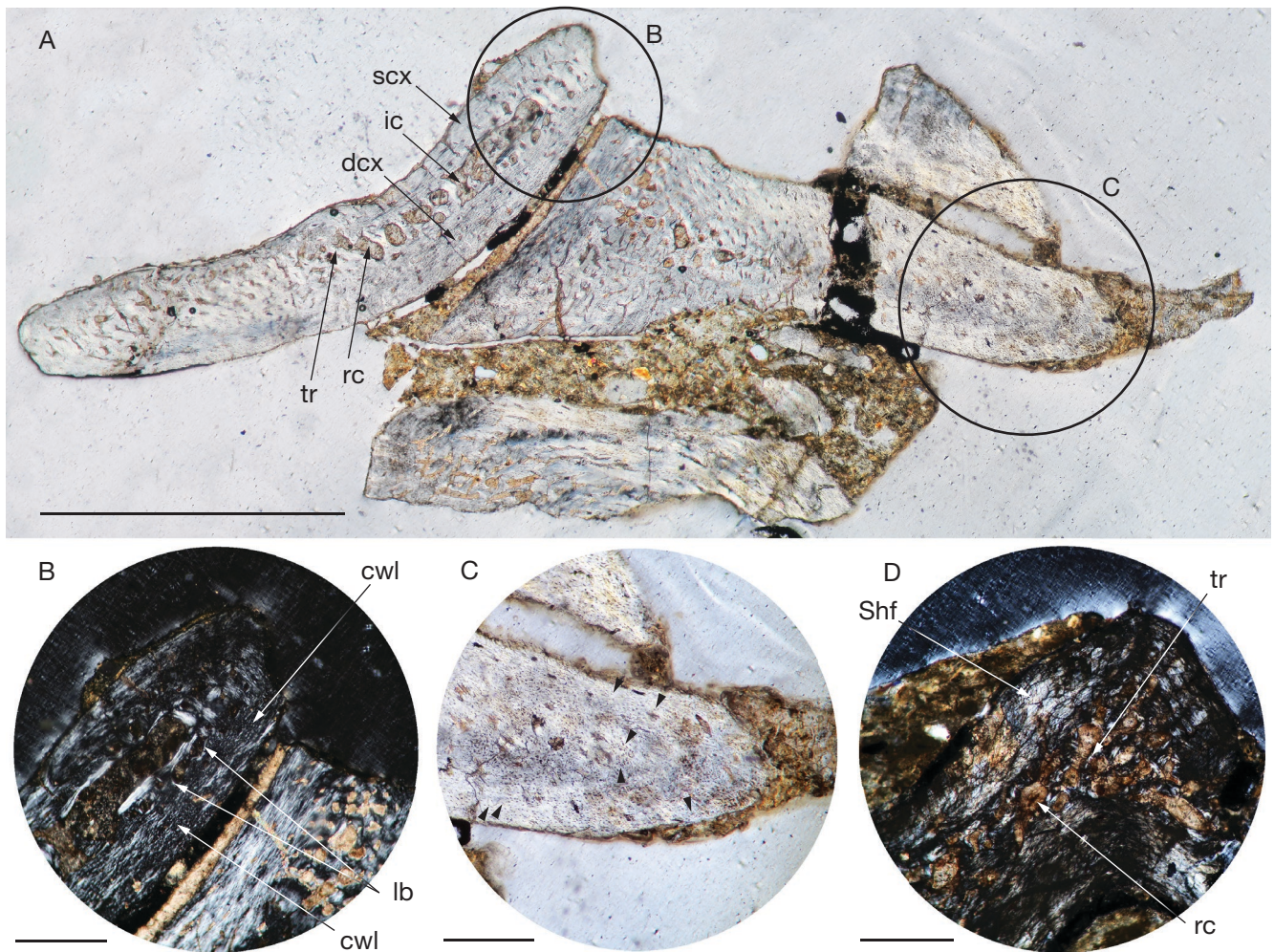
FIG. 9. — Bone histology of the osteoderms of Gracilisuchus stipanicicorum Romer, 1972 (CRILAR PV 490) in A , general view in transversal section of sample G2a under normal light; B , close up of lateral end of the osteoderm marked in A , under polarized light; C , close up of lateral end of the osteoderm marked in A , under normal light; D , close up of the dorsal crest of the sample G2d under polarized light. Abbreviations: dcx : deep cortex; cwl : chicken wire-like structures; ic : inner cancellous core; lb : lamellar bone; rc : resorption cavities; scx : superficial cortex; Shf : Sharpey's fibres; tr : trabecula. Arrowheads indicate osteocyte lacunae. Scale bars: A, 25 mm; B, D, 5 mm and C, 10 mm.
