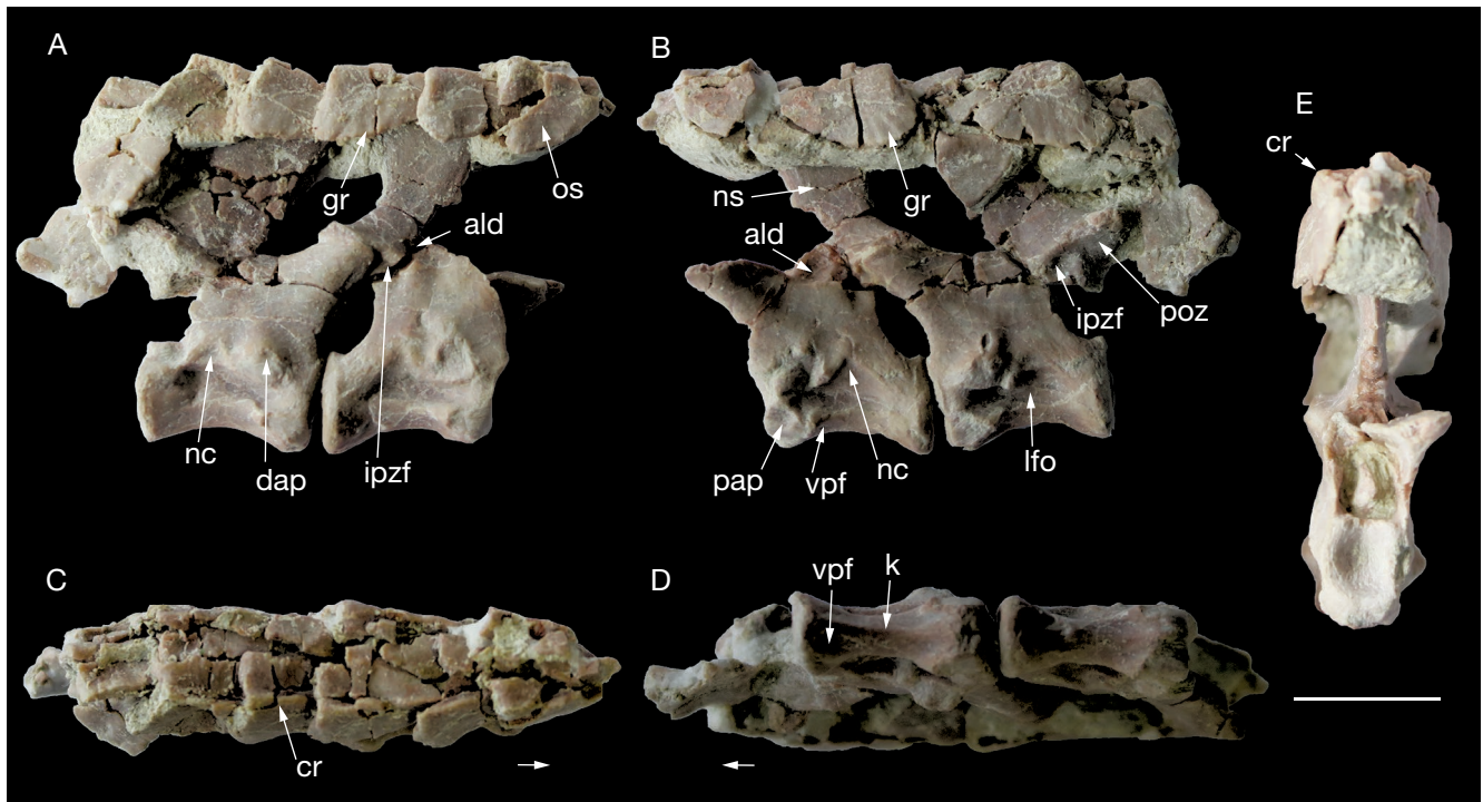
Fig. 3. — Mid cervical vertebrae of Gracilisuchus stipanicorum Romer, 1972 (CRILAR PV 490) in A , right lateral view; B , left lateral view; C , dorsal view; D , ventral view; E , anterior view. Abbreviations: ald : anterolateral depression; cr : dorsal osteoderm crest; dap : diapophysis; gr : groove in osteoderms; ipzf : infrapostzygapophyseal depression; k : keel; lfo : longitudinal lateral fossa on vertebral centrum; nc : inverted V-shaped notch in vertebral centra; ns : neural spine; os : osteoderm; pap : parapophysis; poz : postzygapophysis; vpf : ventral parapophyseal fossa. Arrows indicate anterior direction. Scale bar: 10 mm.
