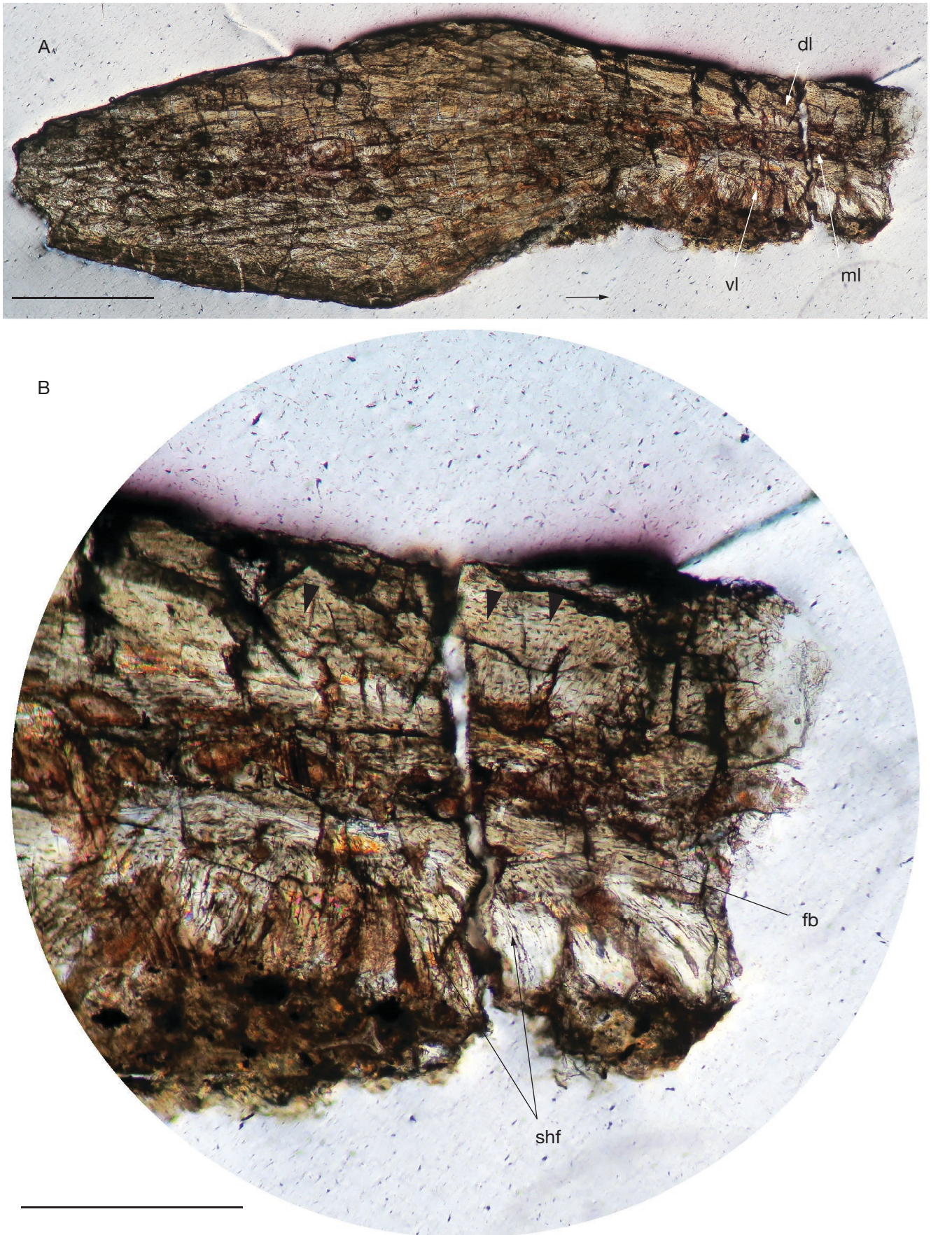
FIG. 10. — Bone histology of an osteoderm of Gracilisuchus stipanichorum Romer, 1972 (CRILAR PV 490) in longitudinal section, sample G4. A , General view under normal light; B , close up of anterior region of the osteoderm in A . Abbreviations: dl : dorsal layer; fb : fibres; ml : middle layer; shf : Sharpey's fibres; vl : ventral layer. Arrowheads indicate osteocyte lacunae, arrow indicates anterior direction. Scale bars: 10 mm ( A ) and 5 mm ( B ).
