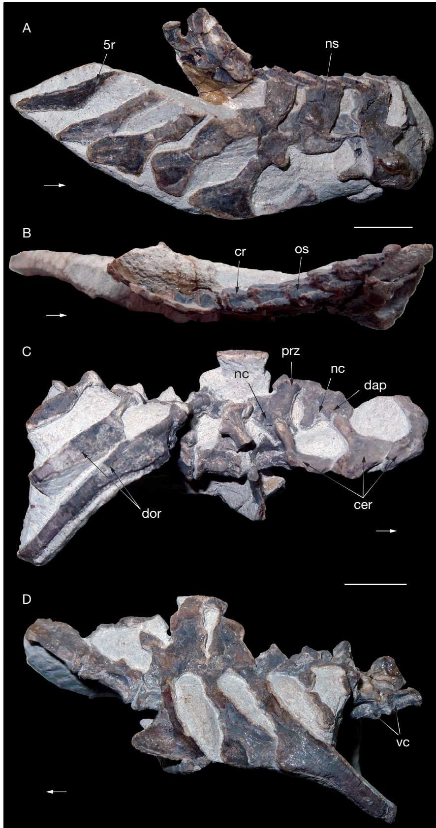
FIG. 2. — Vertebrae of Gracilisuchus stipanicorum Romer, 1972 (CRILAR PV 480), mid cervical vertebrae and 1 st to 5 th preserved ribs in A , right lateral view; B , dorsal view. Fragmentary cervico-dorsal vertebrae in C , right lateral view; D , left lateral view. Abbreviations: 5r : fifth preserved rib; cer : cervical ribs; cr : dorsal osteoderm crest; dap : diapophysis; dor : dorsal ribs; nc : inverted V-shaped notch in vertebral centra; ns : neural spine; os : osteoderm; prz : prezygapophysis; vc : vertebral centra. Arrows indicate anterior direction. Scale bars: 10 mm.
