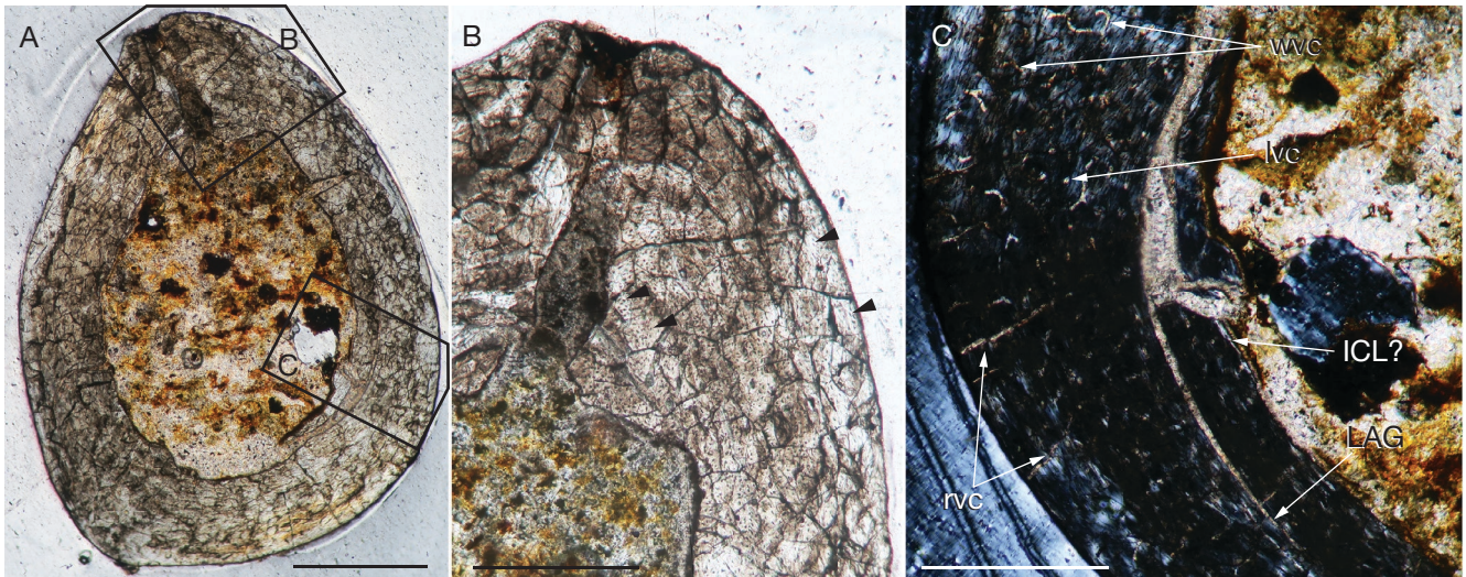
FIG. 8. — Bone histology of the femur of Gracilisuchus stipanicorum Romer, 1972 (CRILAR PV 490) in A , general view of the mid diaphysis cross section under normal light; B , close up of the femoral cortex under normal light; C , close up of the femoral cortex under polarized light. Abbreviations: ICL? : inner circumferential layer?; LAG? : line of arrested growth?; lvc : longitudinal vascular canals; rvc : radial vascular canals; wvc : vermiform vascular canals. Arrowheads indicate osteocyte lacunae. Scale bars: A, 10 mm; B, C, 5 mm.
