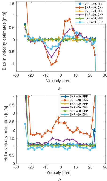
Fig. 9 Velocity error analysis of PPP and DNN for different SNR and \sigma_p = 4 m/s (a) Bias, (b) Std
