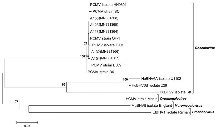
Figure 2 Phylogenetic position of the viral sequences obtained in this work. DPOL gene sequences from representative members of the subfamily Betaherpesvirinae (genera Roseolovirus , Cytomegalovirus , Muromegalovirus and Proboscivirus ) were retrieved from GenBank and RefSeq. PCMV (Suid betaherpesvirus 2/porcine cytomegalovirus): isolate FJ01 (MG696113.1), isolate HN0601 (HQ686081.1), strain B6 (AF268039.2), strain BJ09 (NC_022233.1), strain OF-1 (AF268041.2), strain SC (HQ113116.1). Novel sequences generated in this study: A113 (MN831364), A123 (MN831365), A132 (MN831366), A154 (MN831367), A155 (MN831368). EIBHV1 ( Elephantid betaherpesvirus 1 , NC_020474.2); HCMV ( Human betaherpesvirus 5/human cytomegalovirus , NC_006273.2); HuBHV6A ( Human betaherpesvirus 6A , NC_001664.4); HuBHV6B ( Human betaherpesvirus 6B , NC_000898.1); HuBHV7 ( Human betaherpesvirus 7 , NC_001716.2); MuBHV8 ( Murid betaherpesvirus 8 , NC_019559.1). The evolutionary tree was constructed using the Neighbor-Joining method. The percentage of replicate trees in which the associated taxa clustered together in the bootstrap test (1000 replicates) is shown above the branches (values > 50%). The evolutionary distances were calculated using the Kimura 2-parameter model. There was a total of 173 positions in the final dataset.
