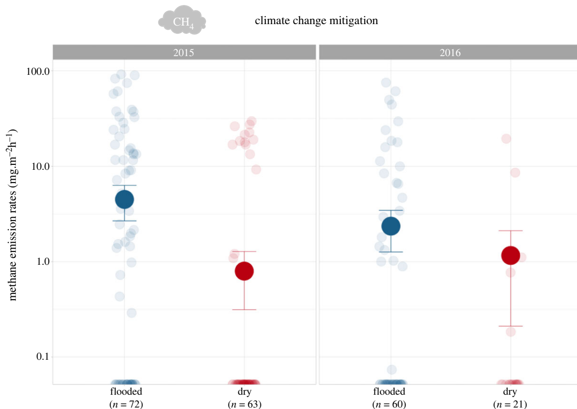
Figure 2. Methane emission rates ( \text{mg m}^{-2} \text{h}^{-1} ) in dry (red points; 2015: n = 63 ; 2016: n = 21 ) and flooded rice fields (blue points; 2015: n = 72 ; 2016: n = 60 ) in the Ebro Delta. Small semi-transparent points indicate observed methane emission rate for each field and fortnightly survey. Large solid points and error bars indicate the estimated emission rate and the standard errors provided by the GLMM, respectively. Note the log-scaled y-axis. (Online version in colour.)
