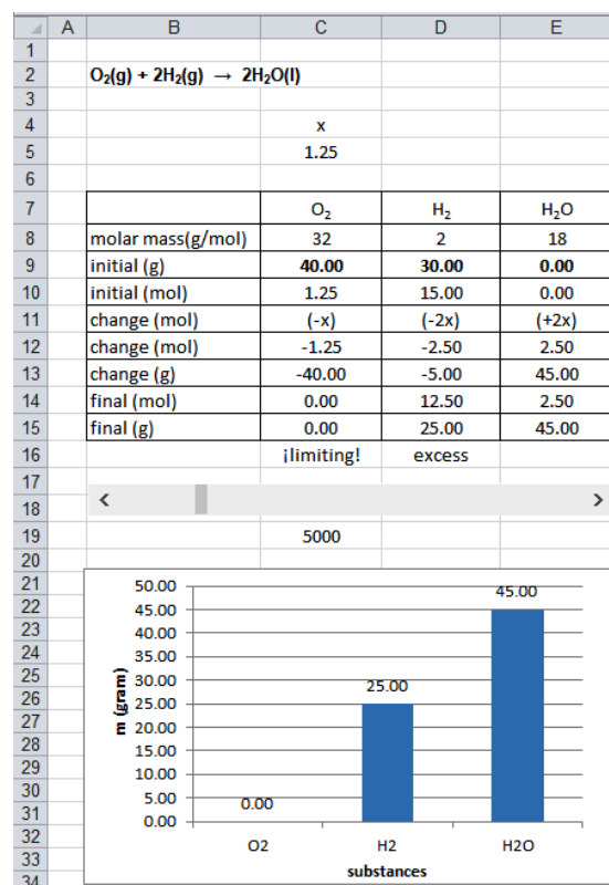
Figure 5. Stoichiometric simulation with masses. The operations carried out are: cell C5: =C19/4000, cell C10: = C9/C8, cell D10: =D9/D8, cell E10: =E9/E8, cell C12: = -C5, cell D12: =-2*C5, cell E12: =2*C5, cell C13: =C12*C8, cell D13: =D12*D8, cell E13: =E12*E8, cell C14: =C10+C12, cell D14: =D10+D12, cell E14: =E10+E12, cell C15: =C14*C8, cell D15: =D14*D8, cell E15: =E14*E8, cell C16: =IF((C15)<=0;"limiting!";"excess"), cell D16: =IF((D15)<=0;"limiting!";"excess")
