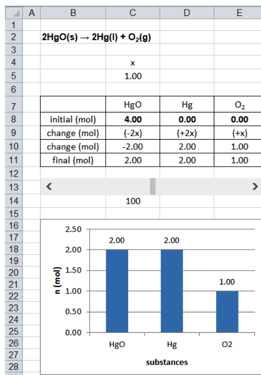
Figure 3. Stoichiometric simulation with moles and graphic representation
